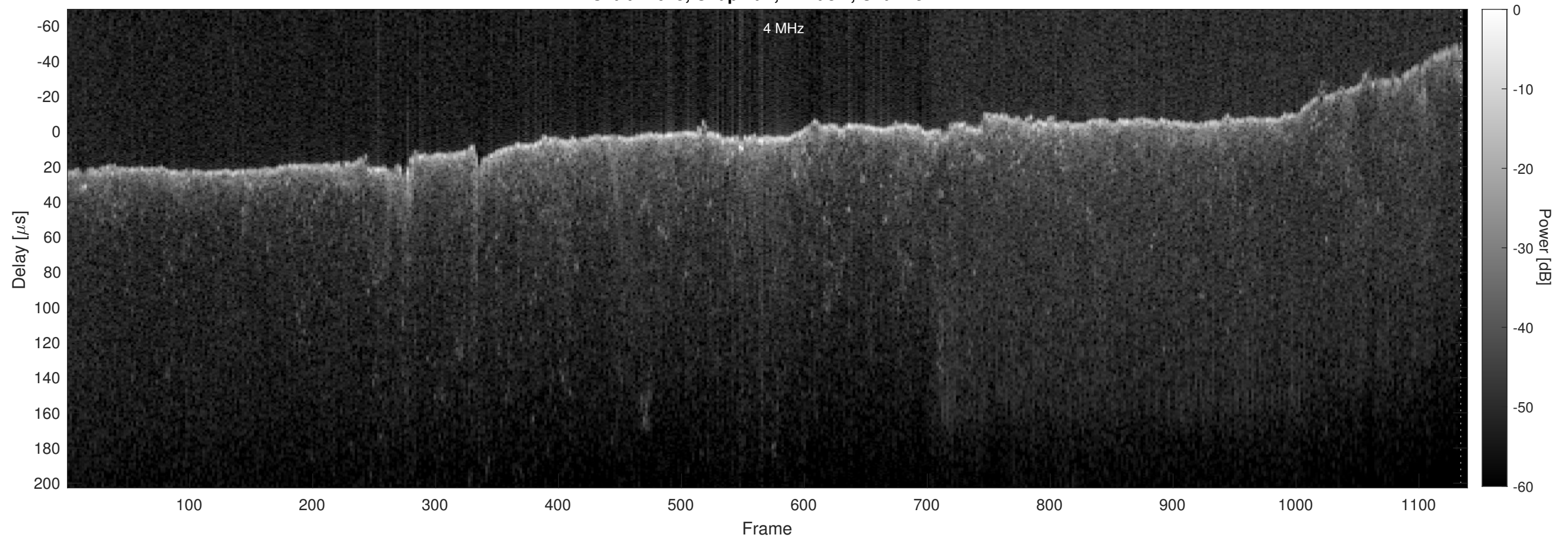
Orbit 21615, Chapman, Window, Channel 2
