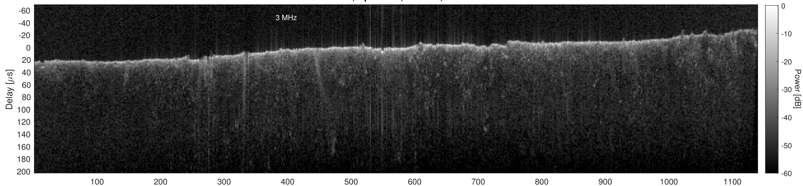
Orbit 21615, Cluttergram
