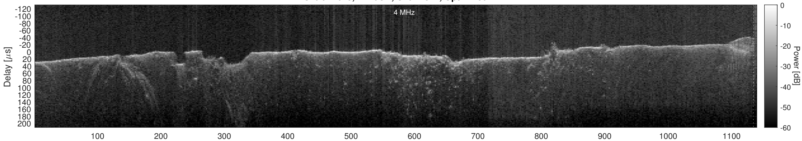
Orbit 21619, Cluttergram
