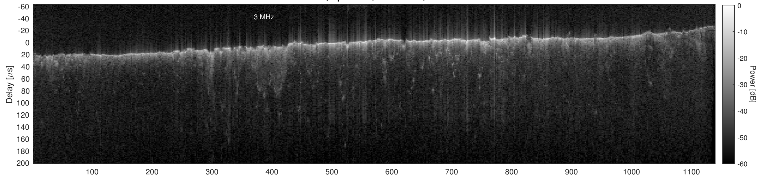
Orbit 21622, Cluttergram
