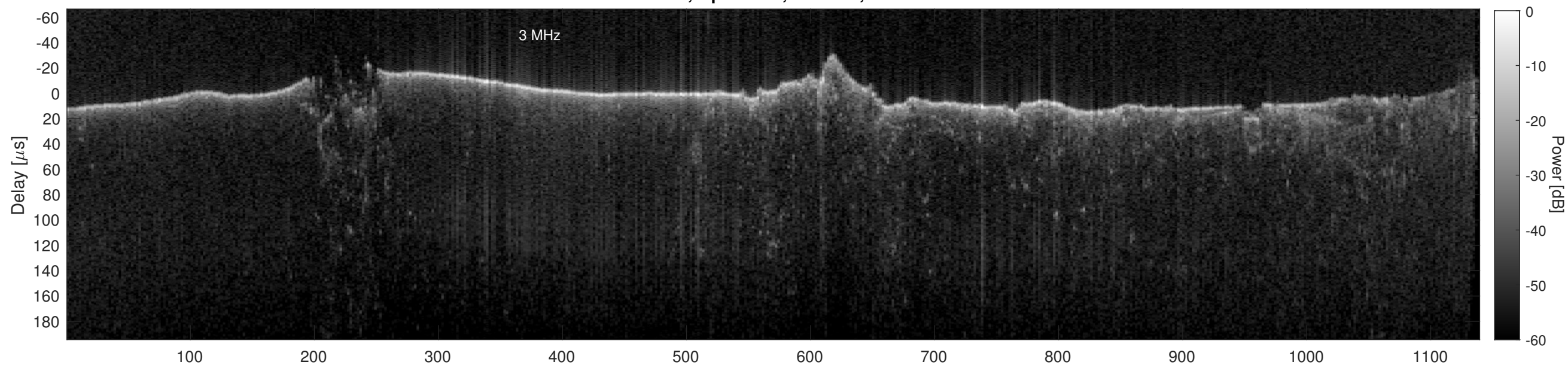
Orbit 21623, Cluttergram
