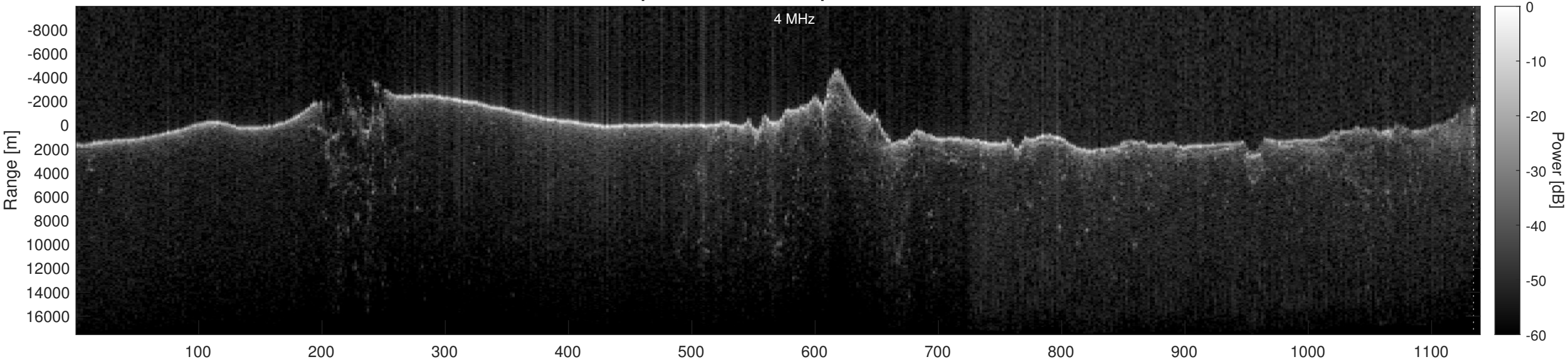
Orbit 21623, Optimized, Window, Depth-Corrected, Channel 2
