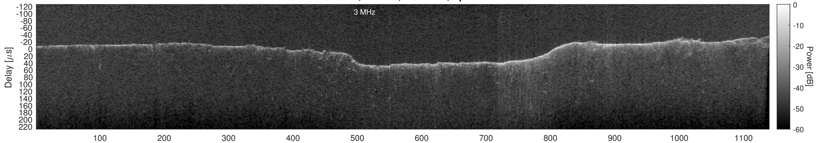
Orbit 21625, Cluttergram
