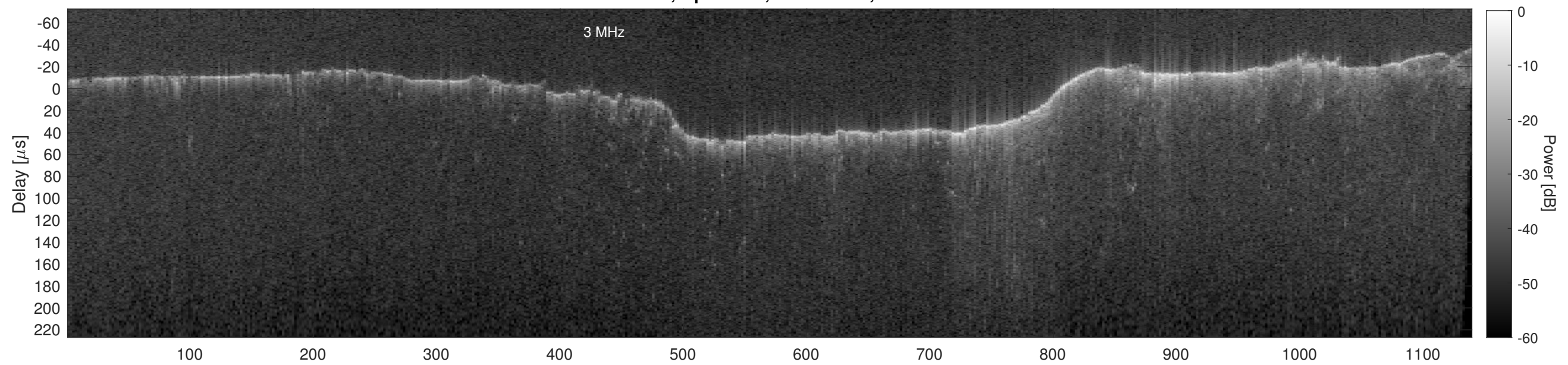
Orbit 21625, Cluttergram
