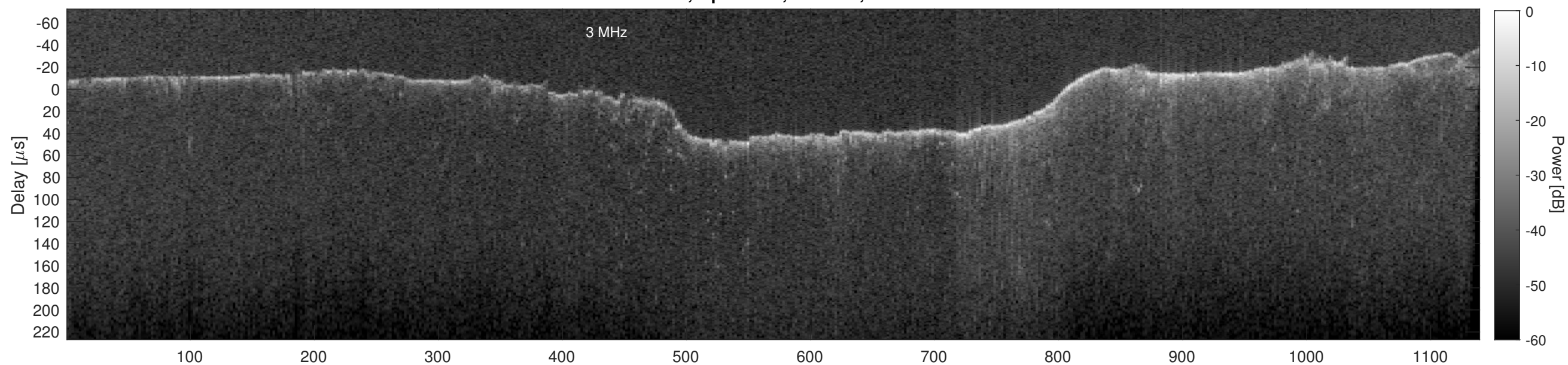
Orbit 21625, Cluttergram
