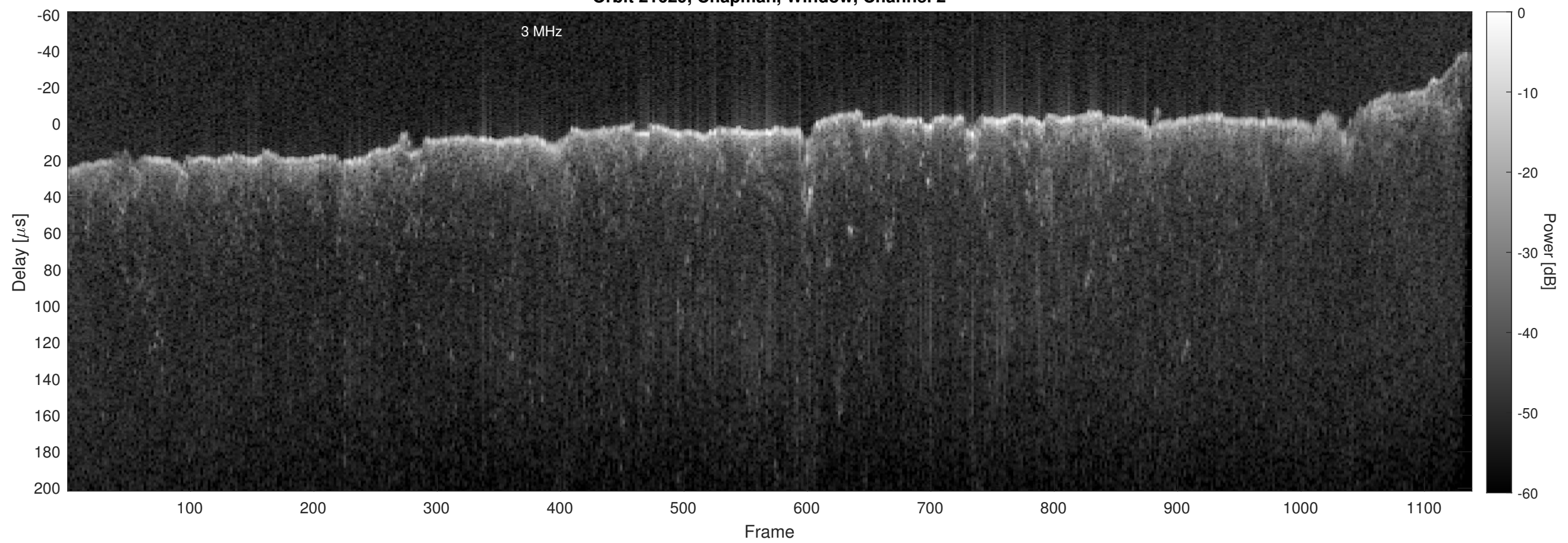
Orbit 21629, Chapman, Window, Channel 2
