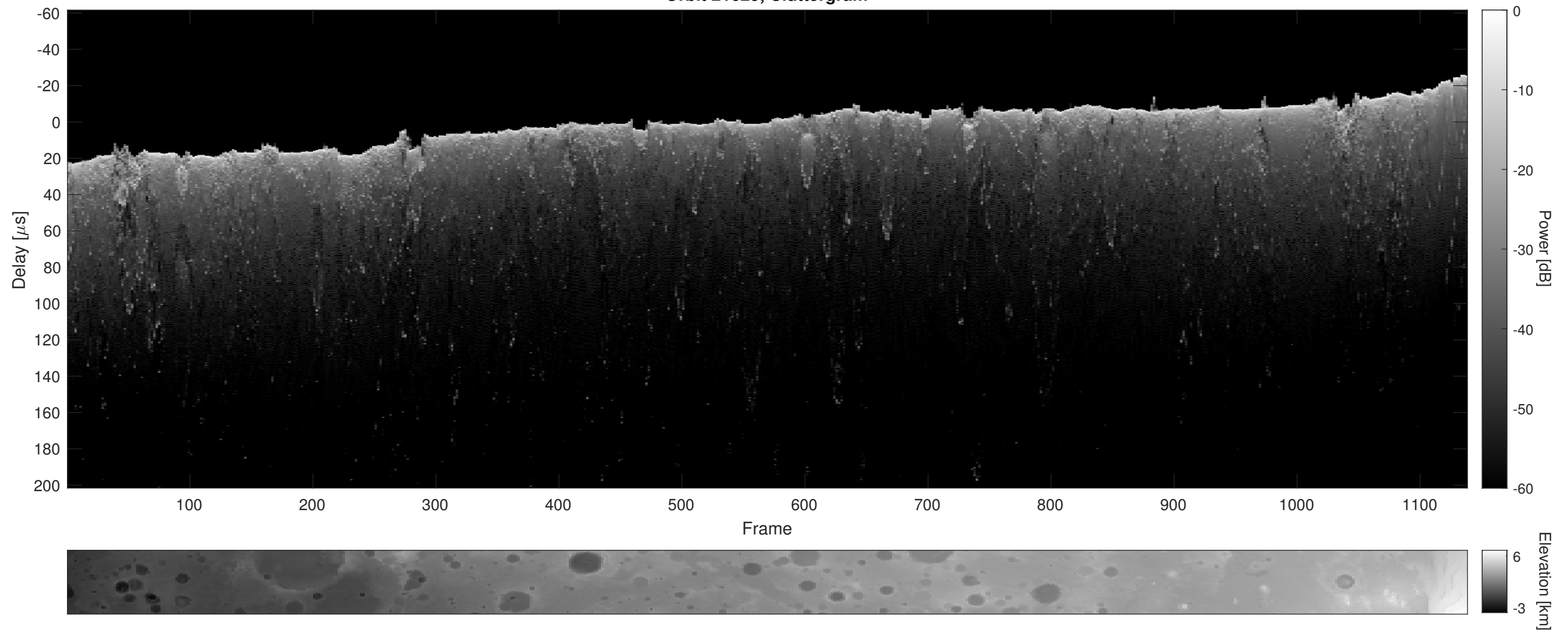
Orbit 21629, Cluttergram
