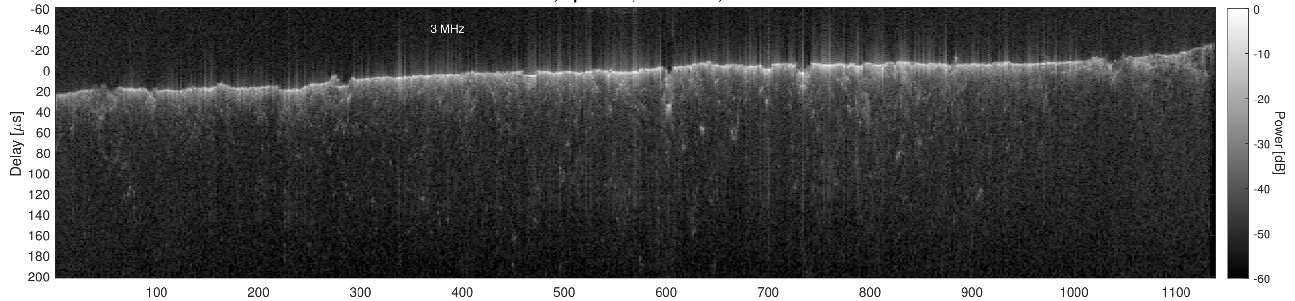
Orbit 21629, Cluttergram
