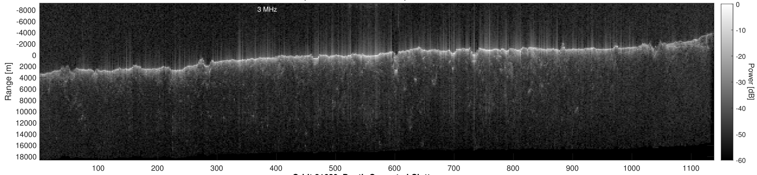
Orbit 21629, Depth-Corrected Cluttergram
