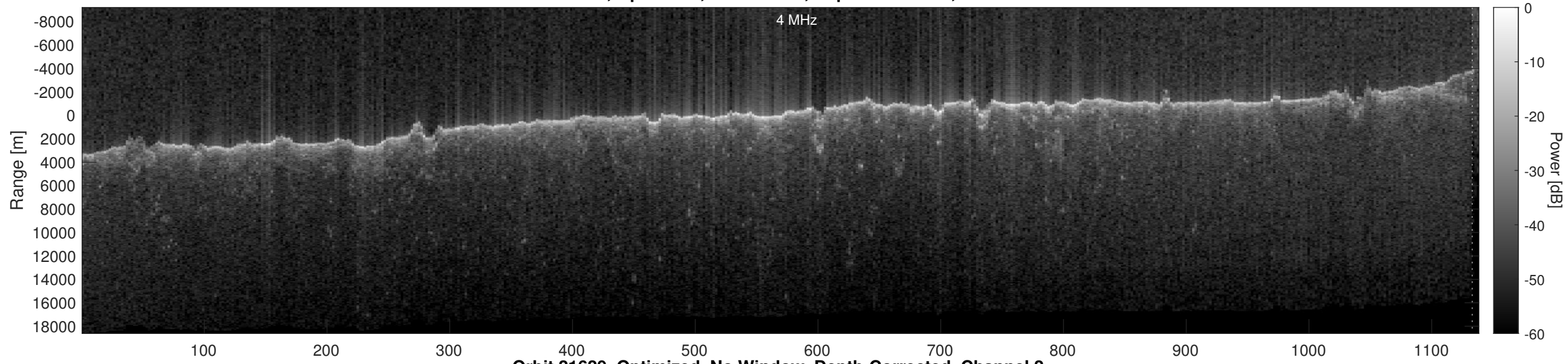
Orbit 21629, Optimized, No Window, Depth-Corrected, Channel 2
