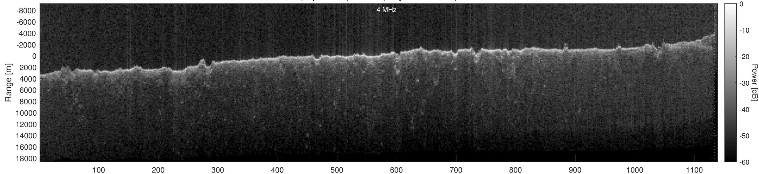
Orbit 21629, Optimized, Window, Depth-Corrected, Channel 2
