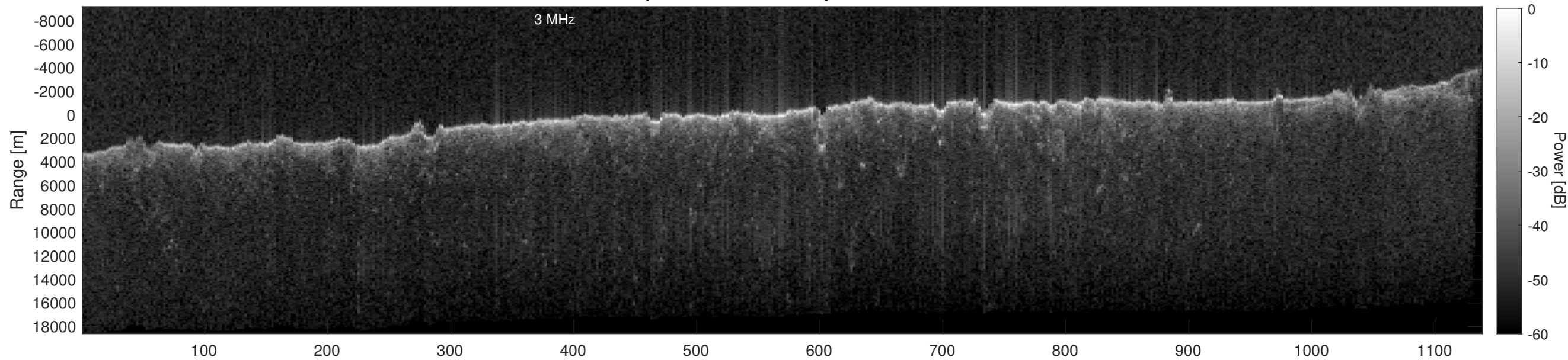
Orbit 21629, Depth-Corrected Cluttergram
