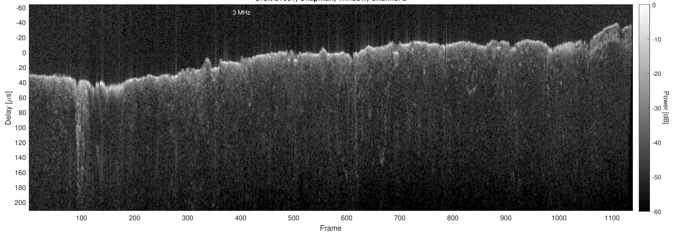
Orbit 21631, Chapman, Window, Channel 2
