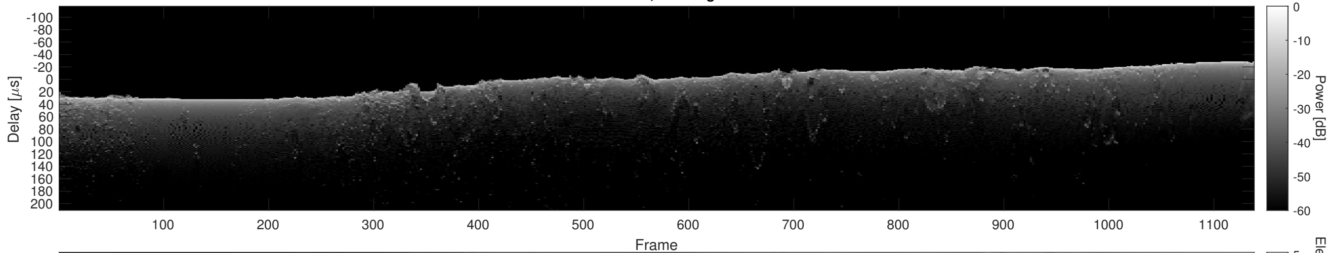
Orbit 21631, Cluttergram
