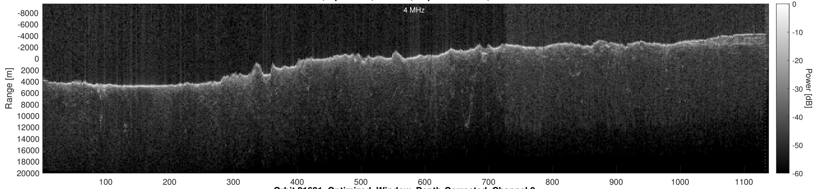
Orbit 21631, Optimized, Window, Depth-Corrected, Channel 2
