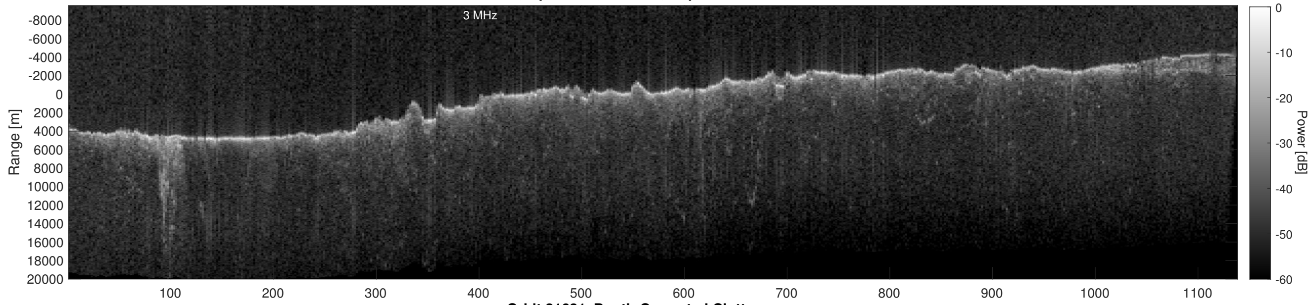
Orbit 21631, Depth-Corrected Cluttergram
