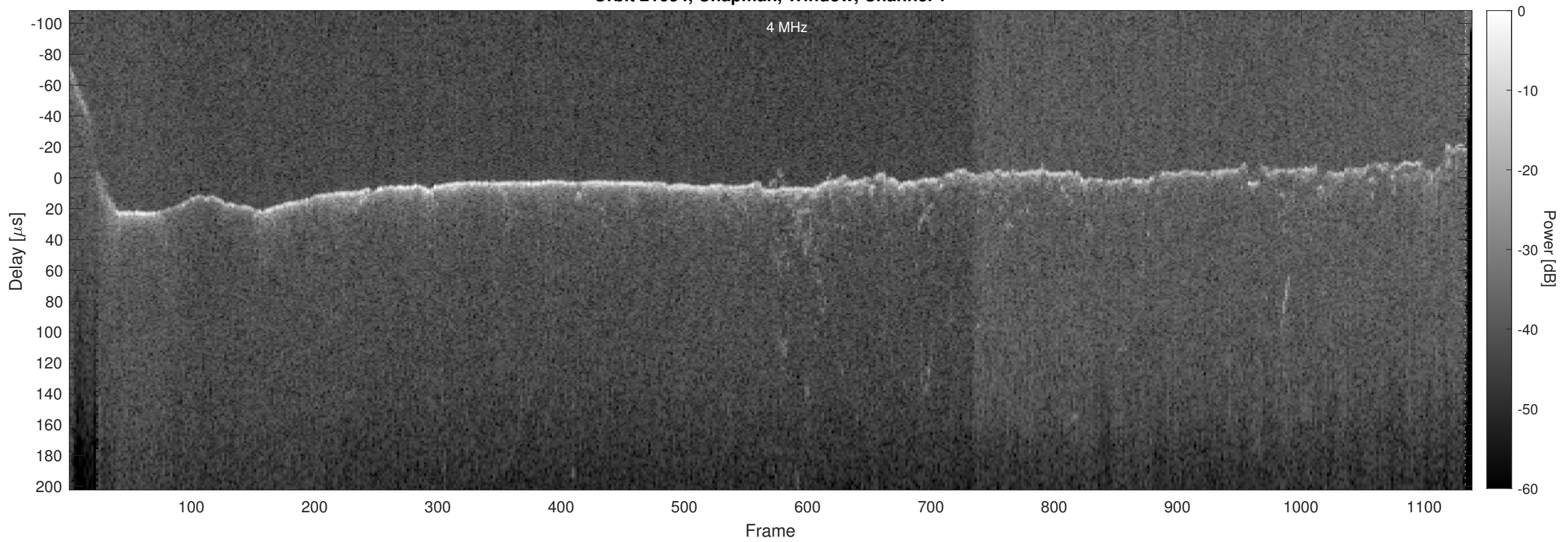
Orbit 21634, Chapman, Window, Channel 2
