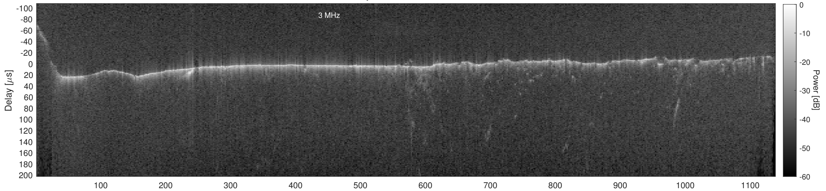
Orbit 21634, Cluttergram
