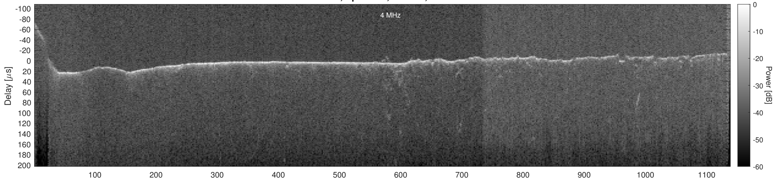
Orbit 21634, Optimized, Window, Channel 2
