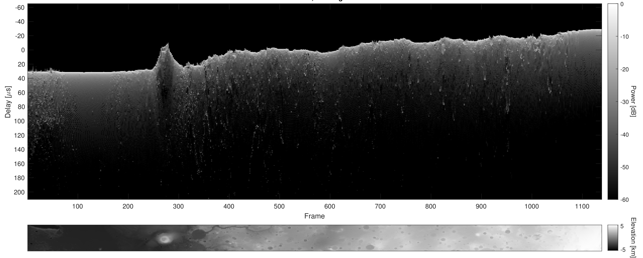
Orbit 21638, Cluttergram
