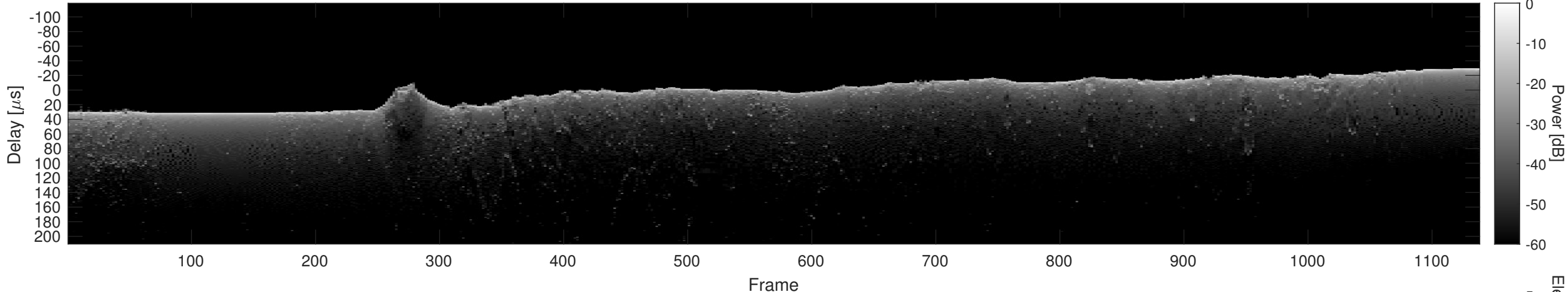
Orbit 21638, Cluttergram
