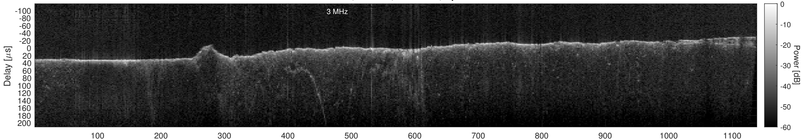
Orbit 21638, Cluttergram
