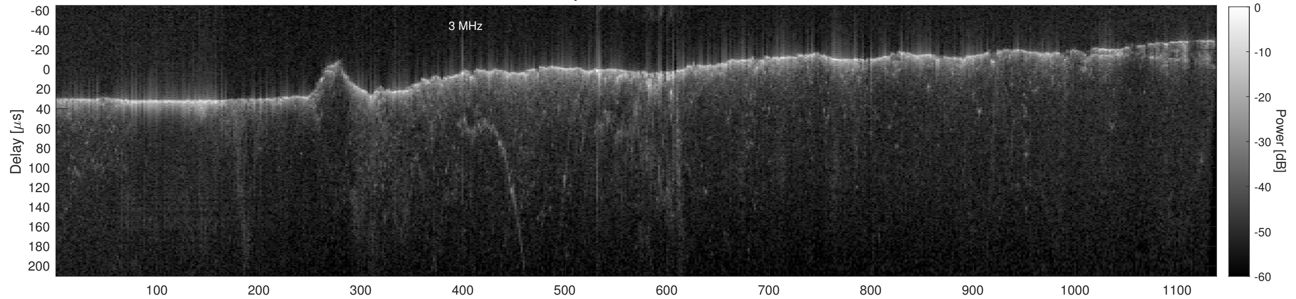
Orbit 21638, Cluttergram
