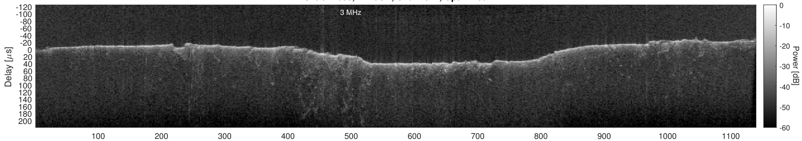
Orbit 21639, Cluttergram
