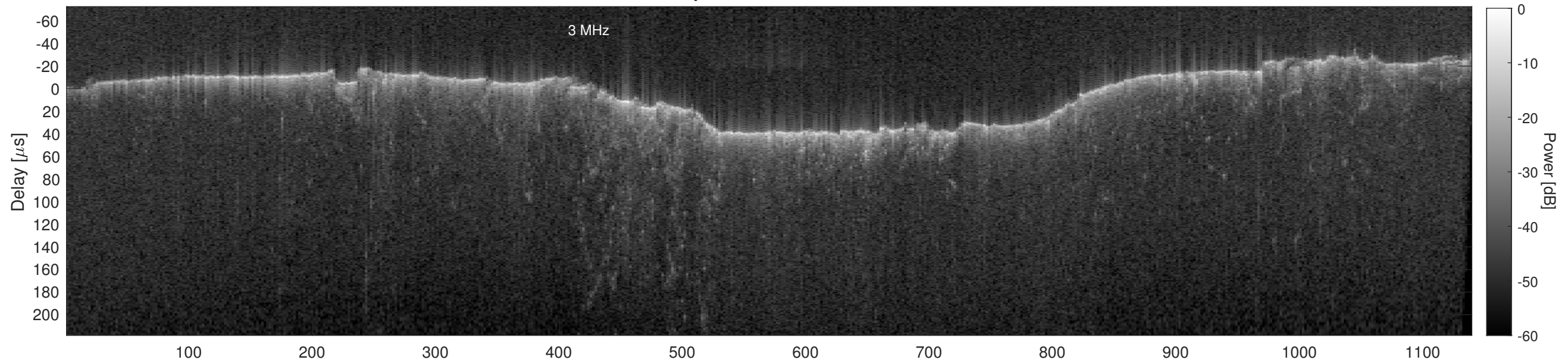
Orbit 21639, Cluttergram
