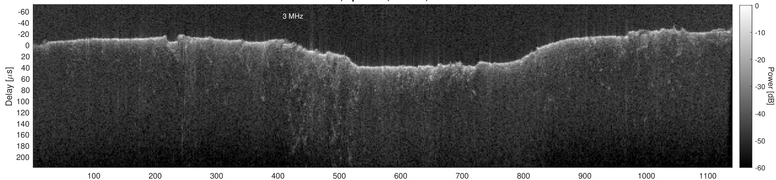
Orbit 21639, Cluttergram
