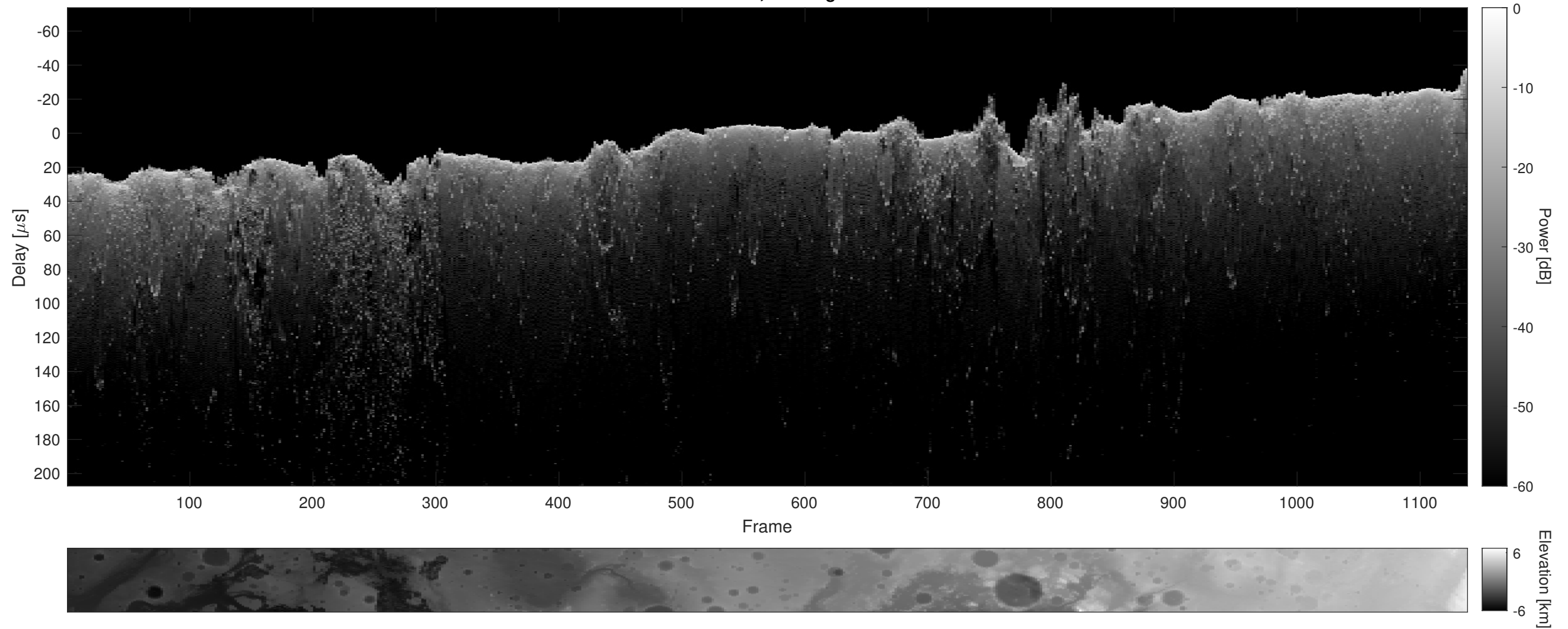
Orbit 21640, Cluttergram
