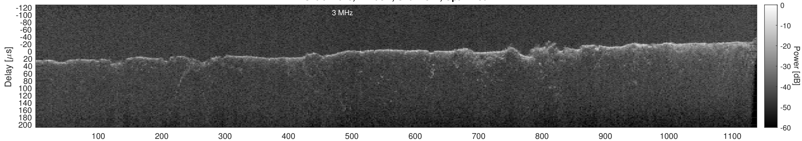
Orbit 21640, Cluttergram
