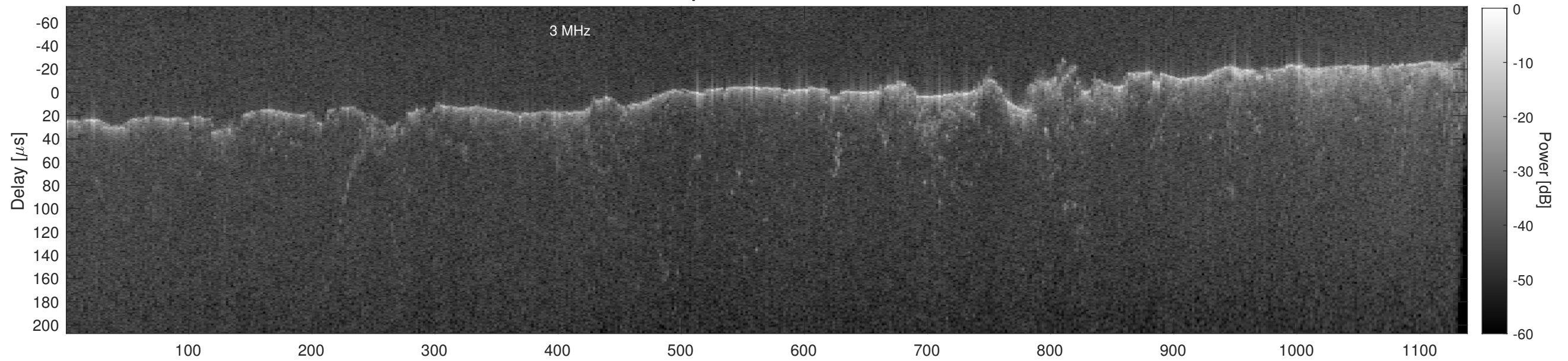
Orbit 21640, Cluttergram
