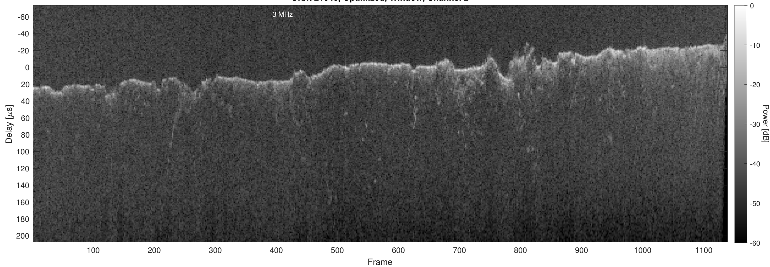
Orbit 21640, Optimized, Window, Channel 2
