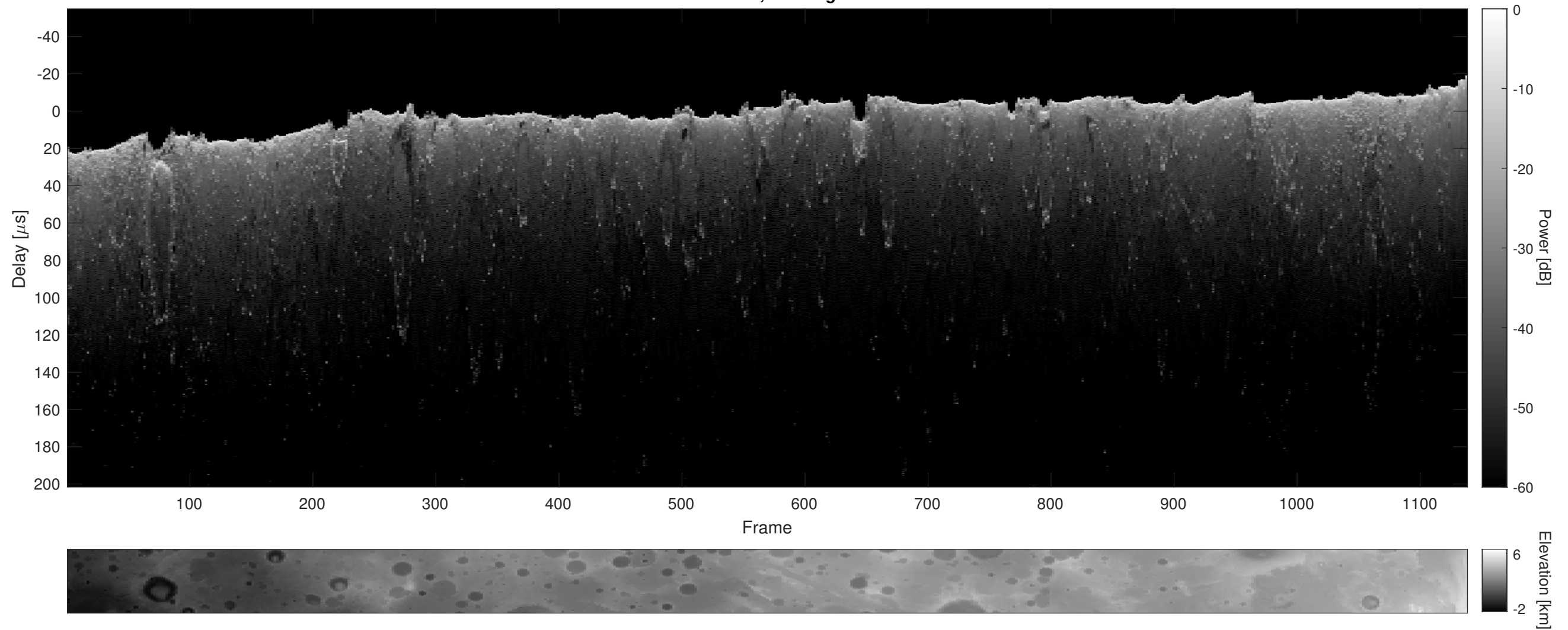
Orbit 21643, Cluttergram
