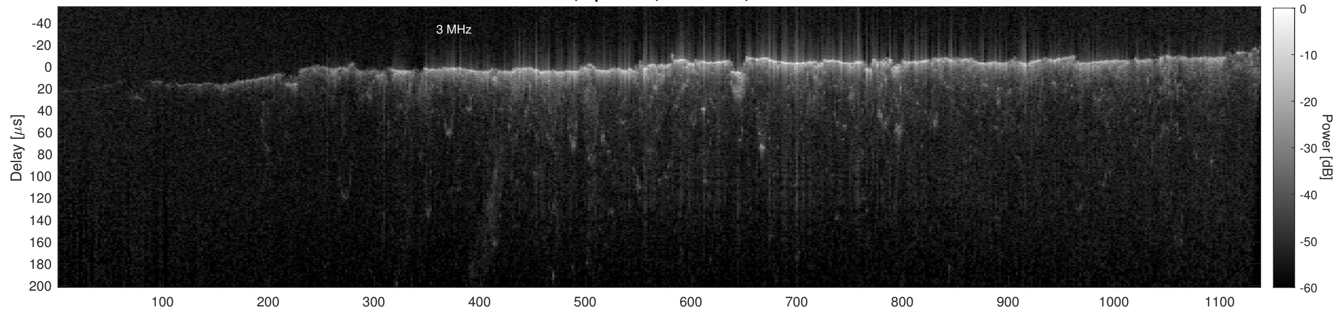
Orbit 21643, Cluttergram
