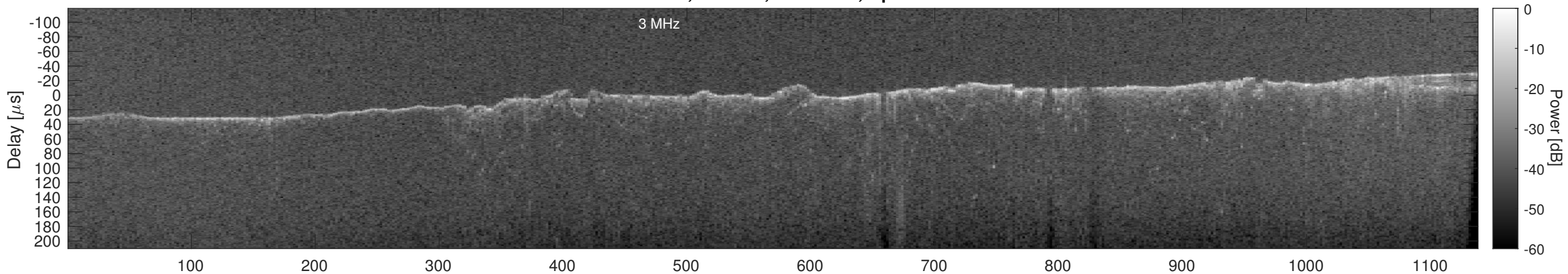
Orbit 21645, Cluttergram
