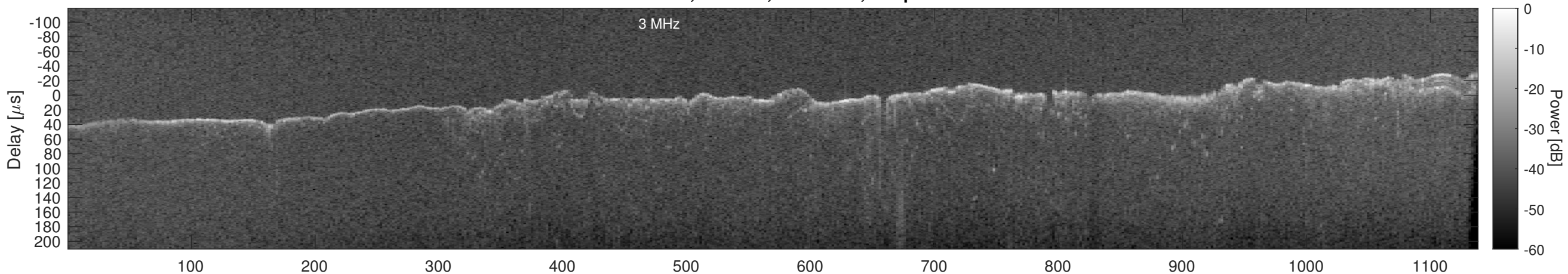
Orbit 21645, Window, Channel 2, Optimized
