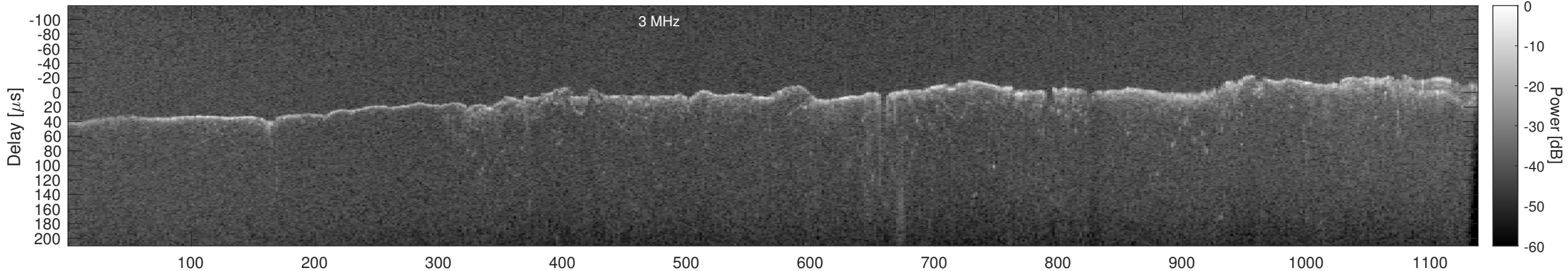
Orbit 21645, Window, Channel 2, Chapman
