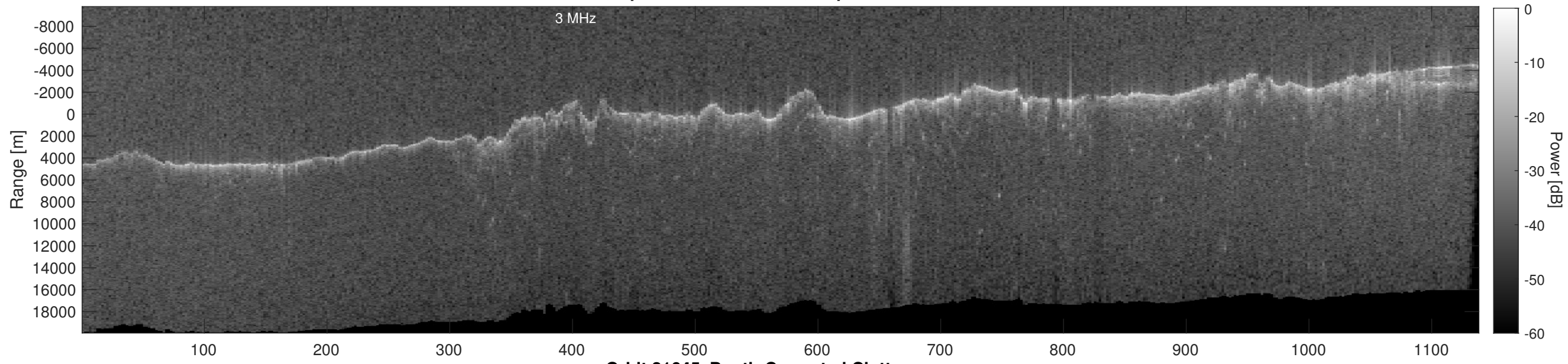
Orbit 21645, Depth-Corrected Cluttergram
