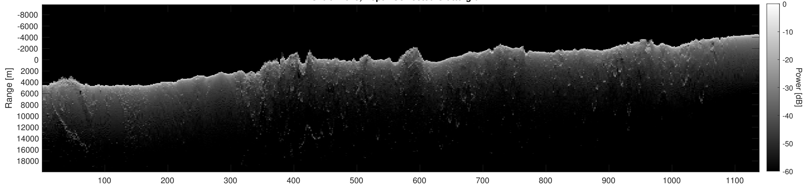
Orbit 21645, Depth-Corrected Cluttergram
