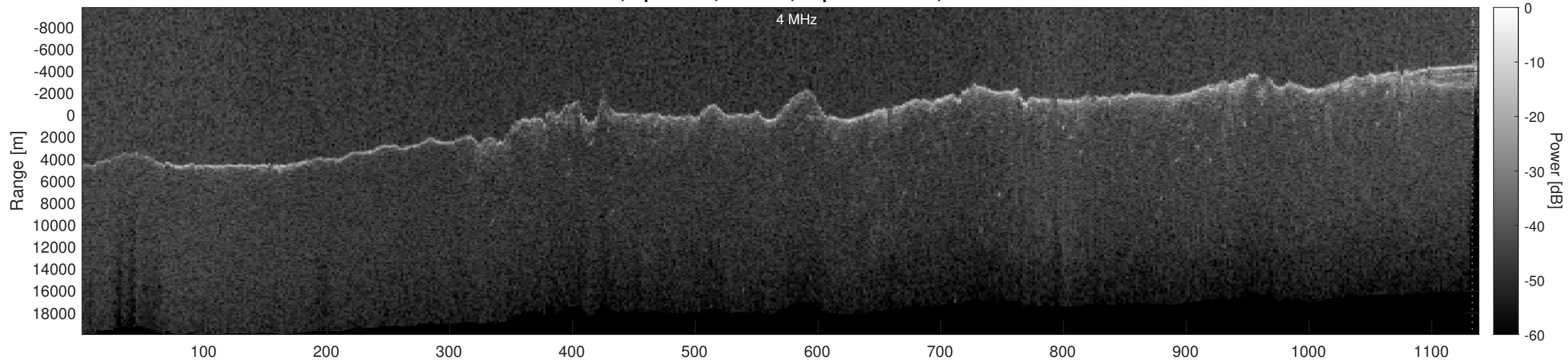
Orbit 21645, Optimized, Window, Depth-Corrected, Channel 2
