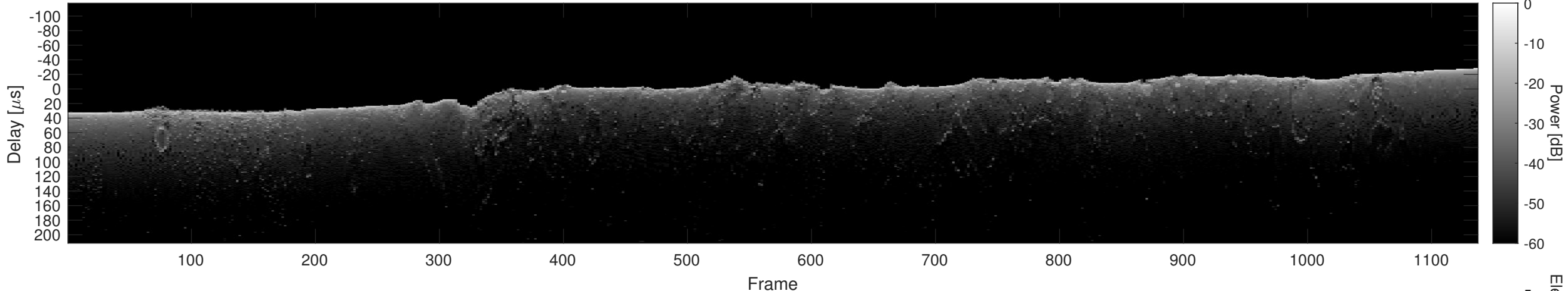
Orbit 21652, Cluttergram
