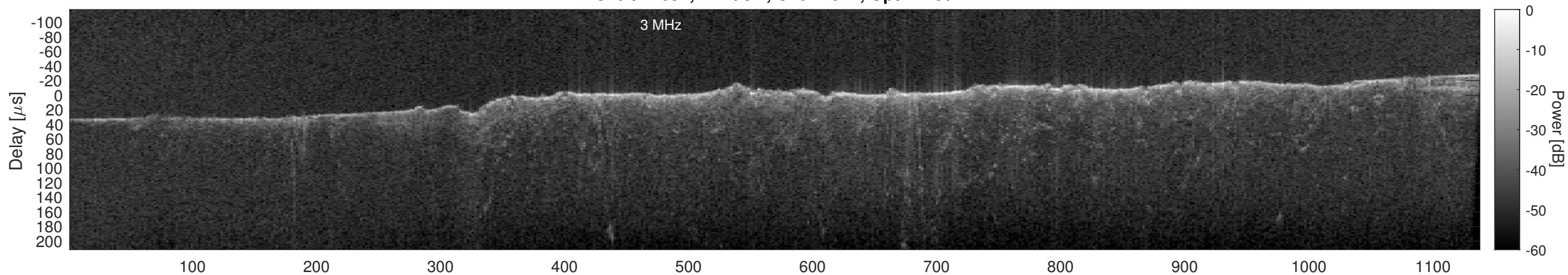
Orbit 21652, Cluttergram
