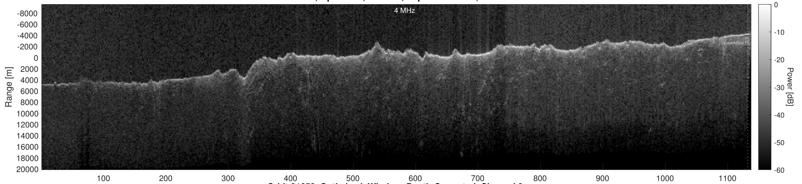
Orbit 21652, Optimized, Window, Depth-Corrected, Channel 2
