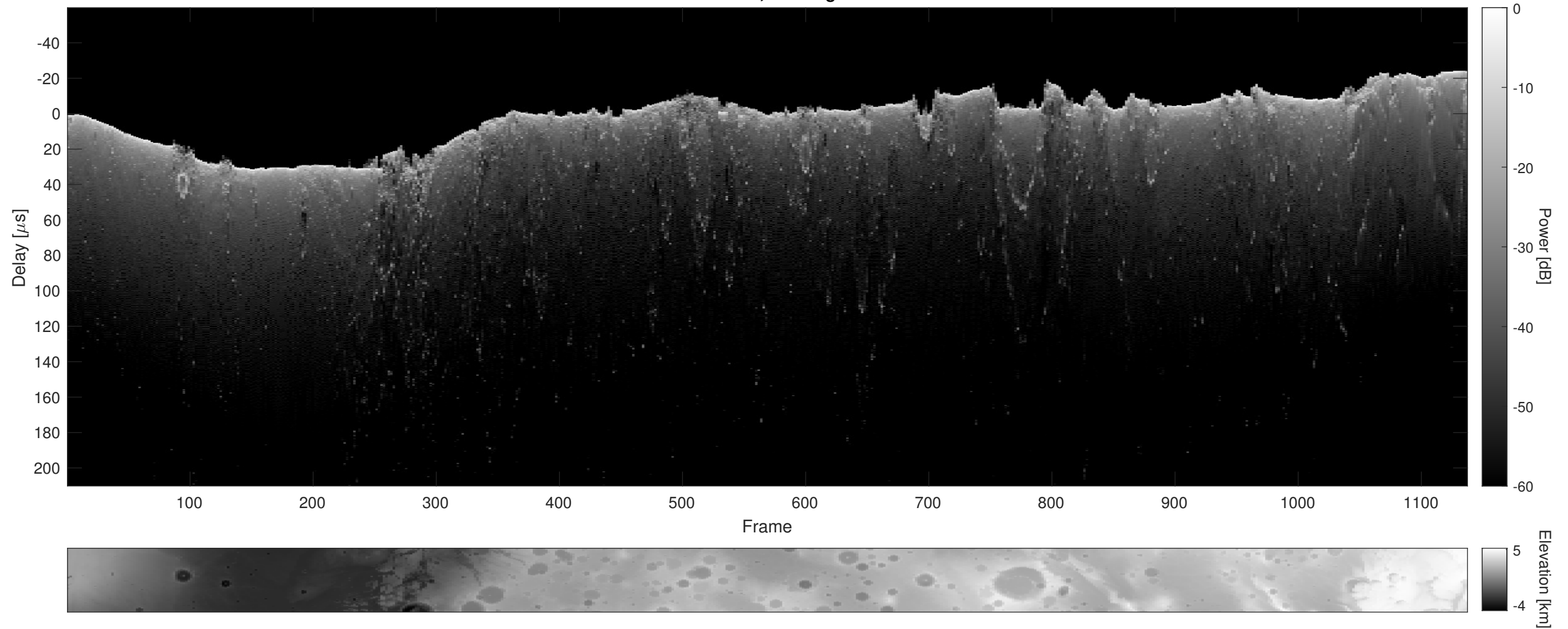
Orbit 21663, Cluttergram
