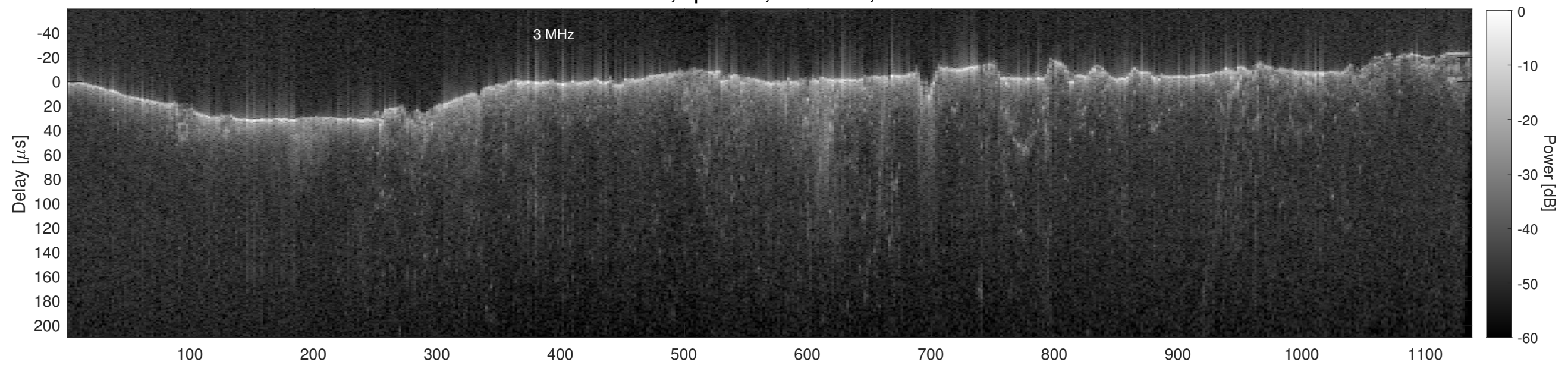
Orbit 21663, Cluttergram
