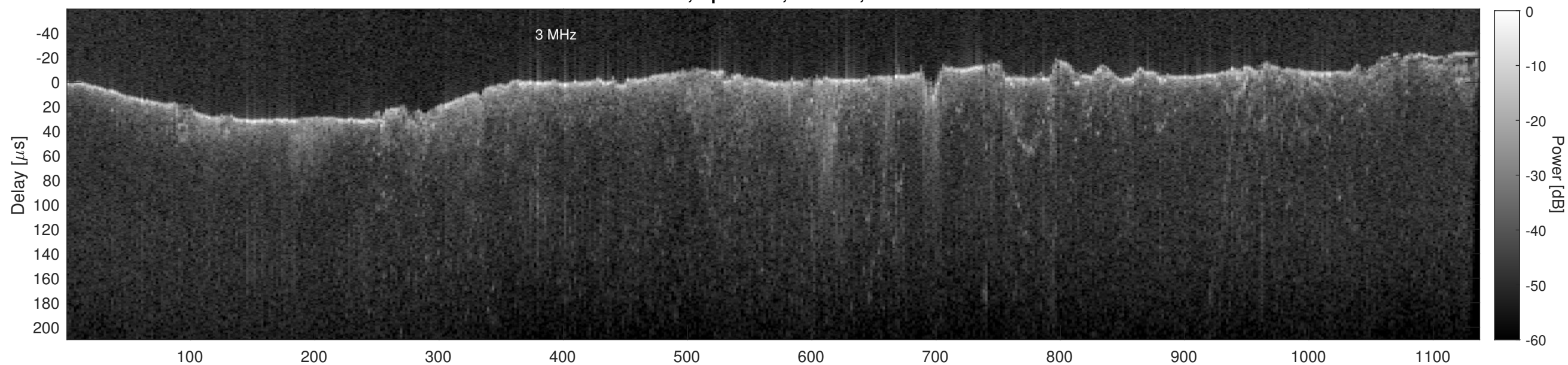
Orbit 21663, Cluttergram
