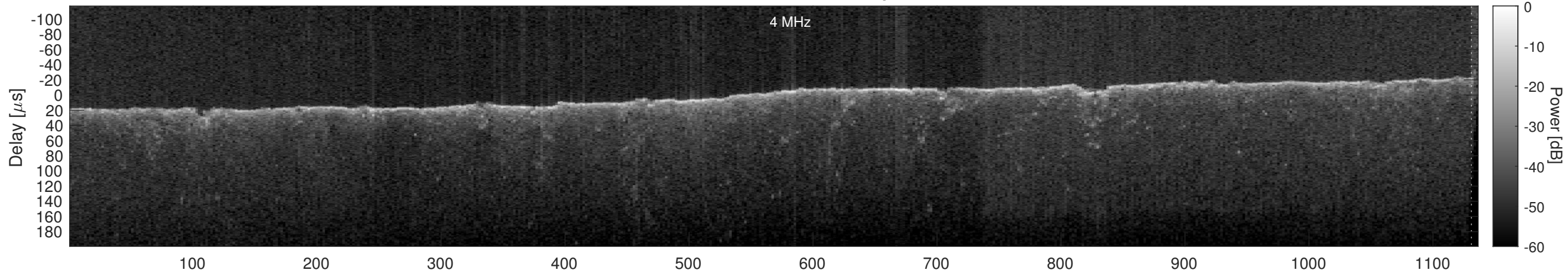
Orbit 21675, Cluttergram
