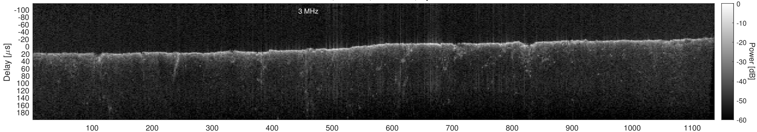
Orbit 21675, Cluttergram
