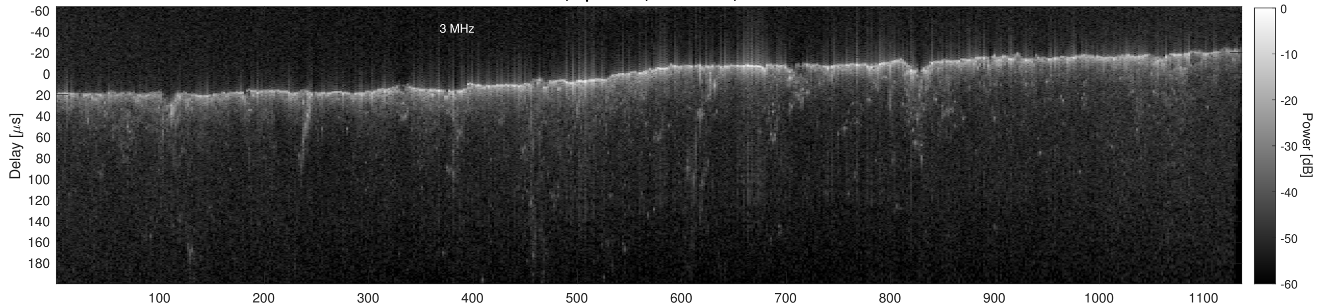
Orbit 21675, Cluttergram
