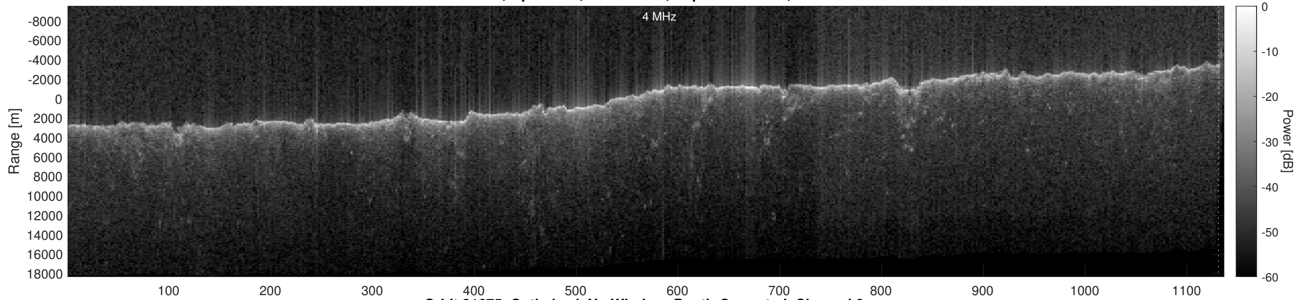
Orbit 21675, Optimized, No Window, Depth-Corrected, Channel 2
