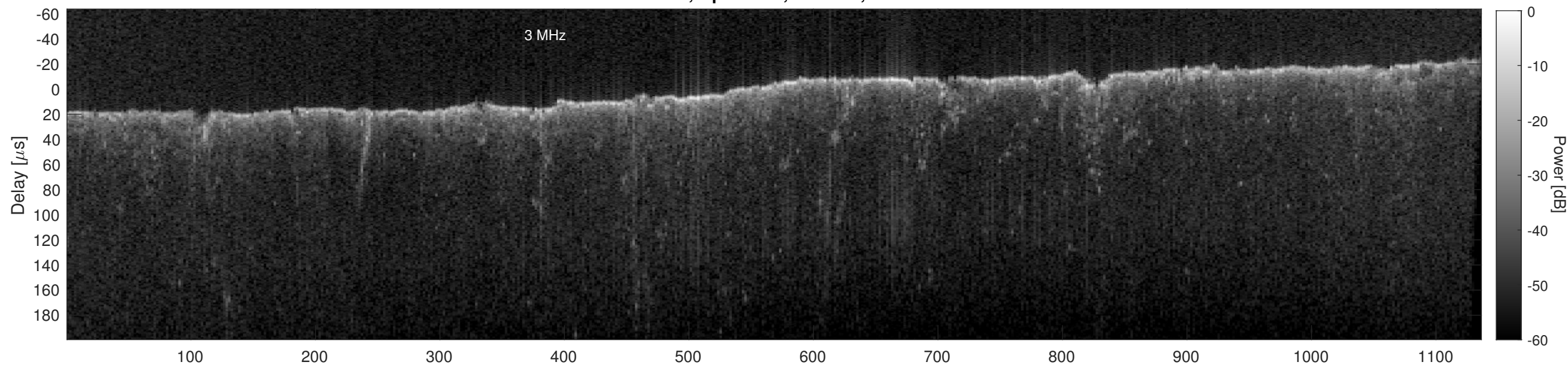
Orbit 21675, Cluttergram
