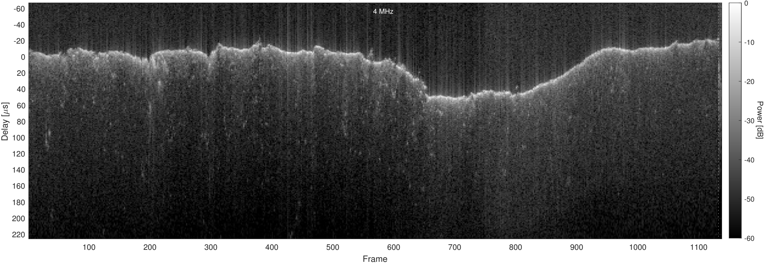
Orbit 21685, Chapman, No Window, Channel 2
