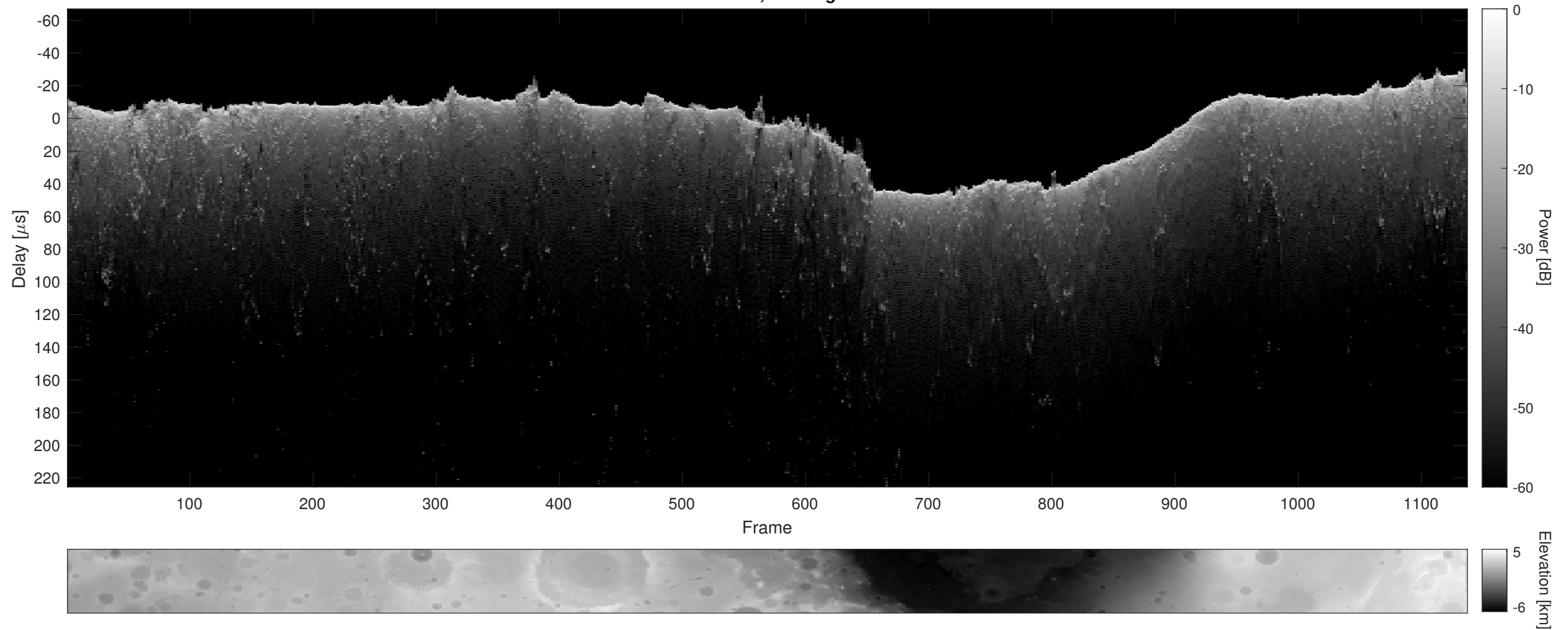
Orbit 21685, Cluttergram
