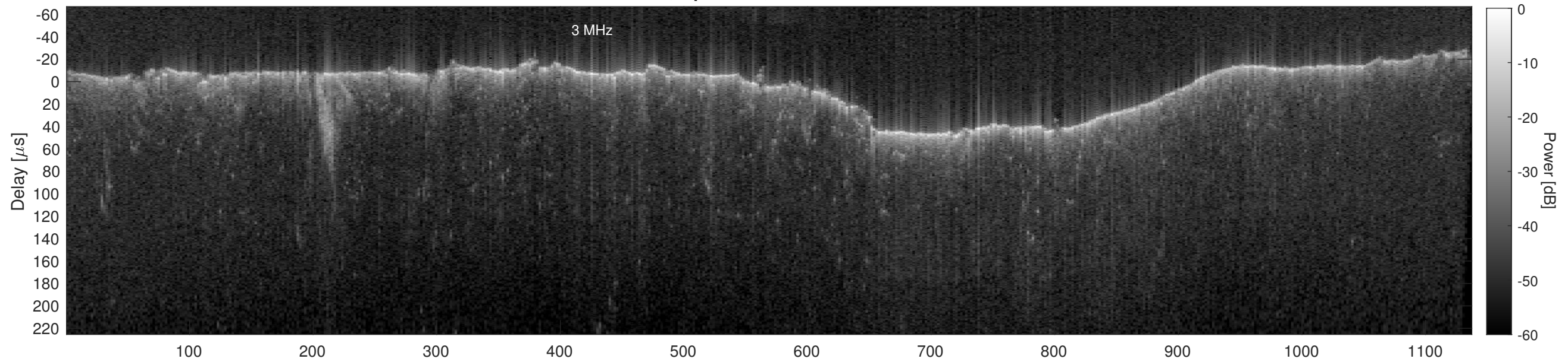
Orbit 21685, Cluttergram
